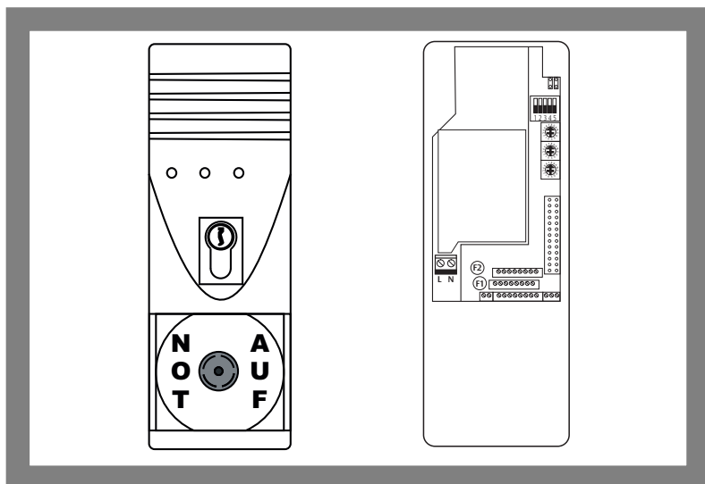
Fig. 1: Escape door control terminal 1338 – open rear side on right
