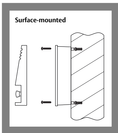
Fig. 4: Wall mount
